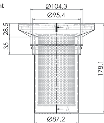
Cross Section
