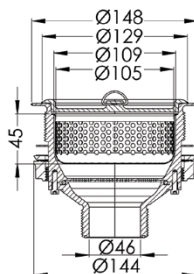
Cross Section
