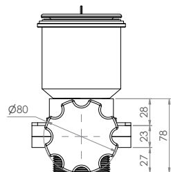
Side
