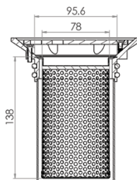
Cross Section
