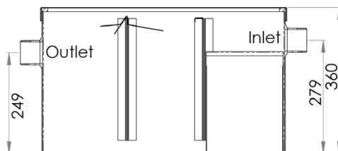
Cross Section
