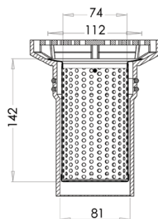
Cross Section
