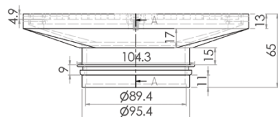
Front
