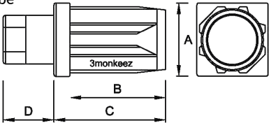
Zinc Die-Cast Chrome Plated Adjustable Hex Foot - Square Tube
