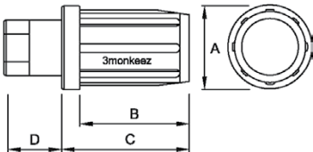
304 Grade Stainless Steel Clad Adjustable Hex Foot - Round Tube
