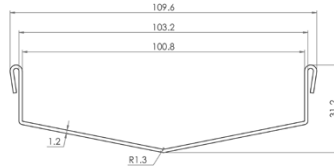
Profile
