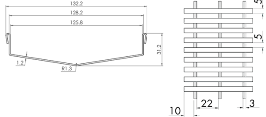
Profile
