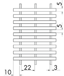
Grate
