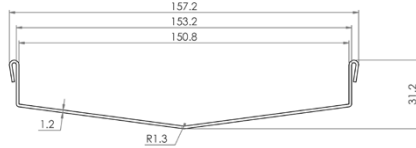
Profile
