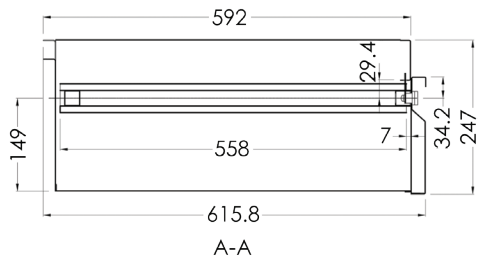
Cross Section
